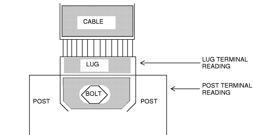
Figure F-7—Single terminal connection (typical)
