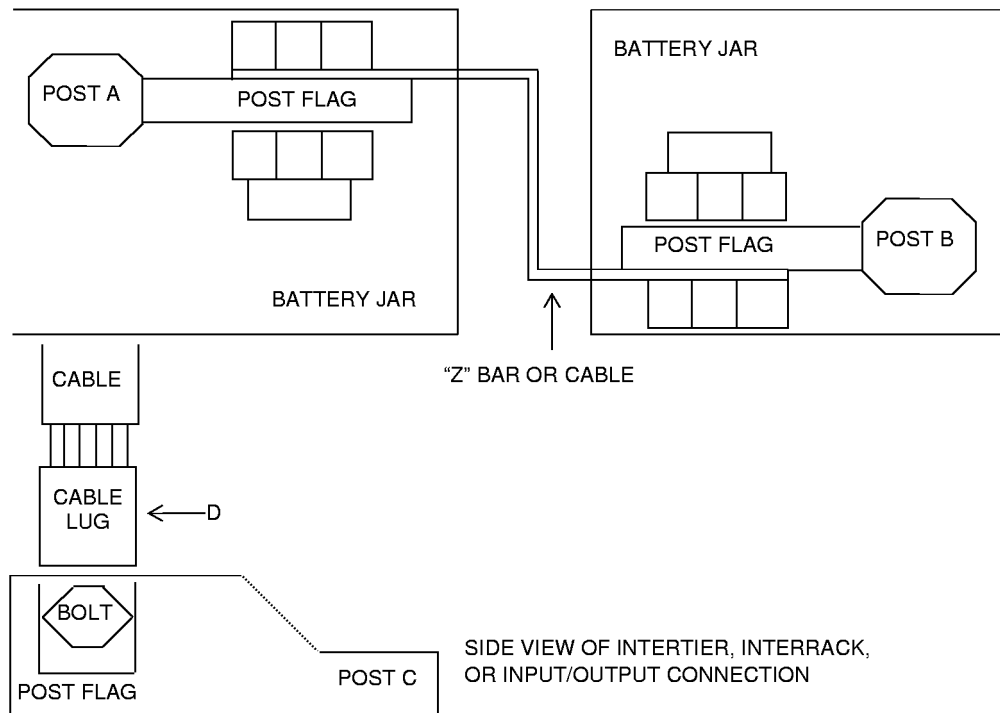
Figure F-6—Flag-post terminal connections (typical)
