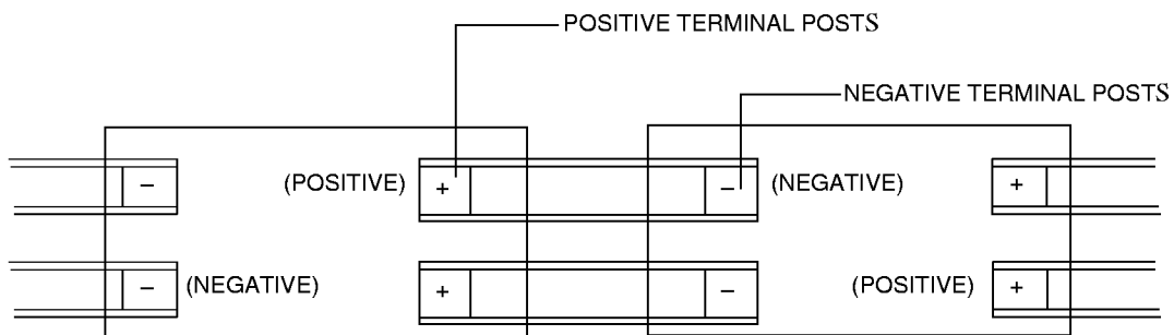
Figure F-3—Parallel-post intercell connection (typical)
