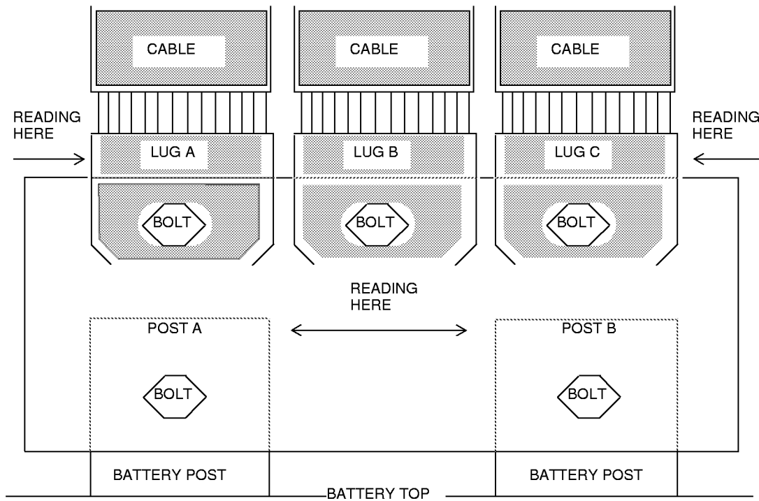
Figure F-9—Cable, plate, and post connections
