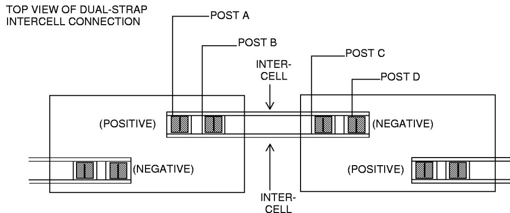
Figure F-4—Double-post intercell connection (typical)
